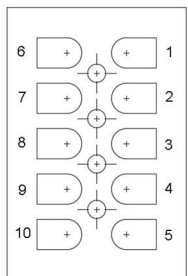
Screw terminals view
