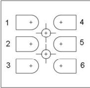
Screw terminal view
